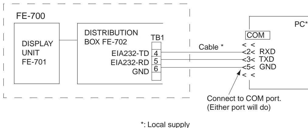
Figure 1 Interconnection between FE-700 and PC
